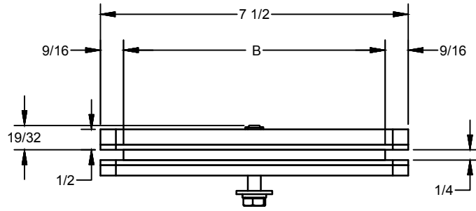
SL SERIES ARBOR THERNS TEE WALL
