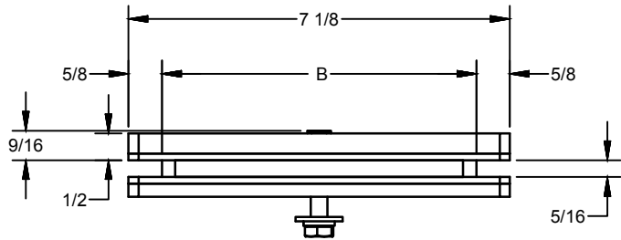
SL SERIES ARBOR STEEL TEE WALL
