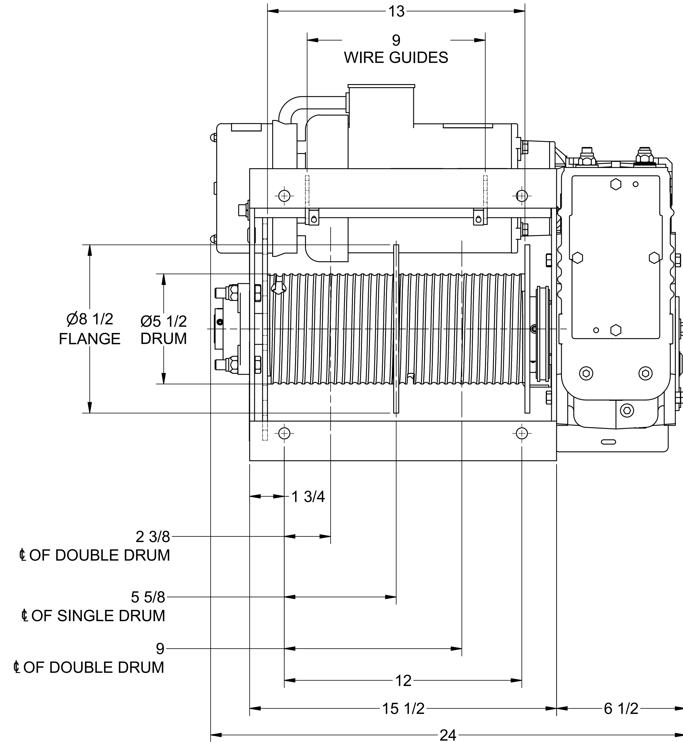
REAR VIEW
