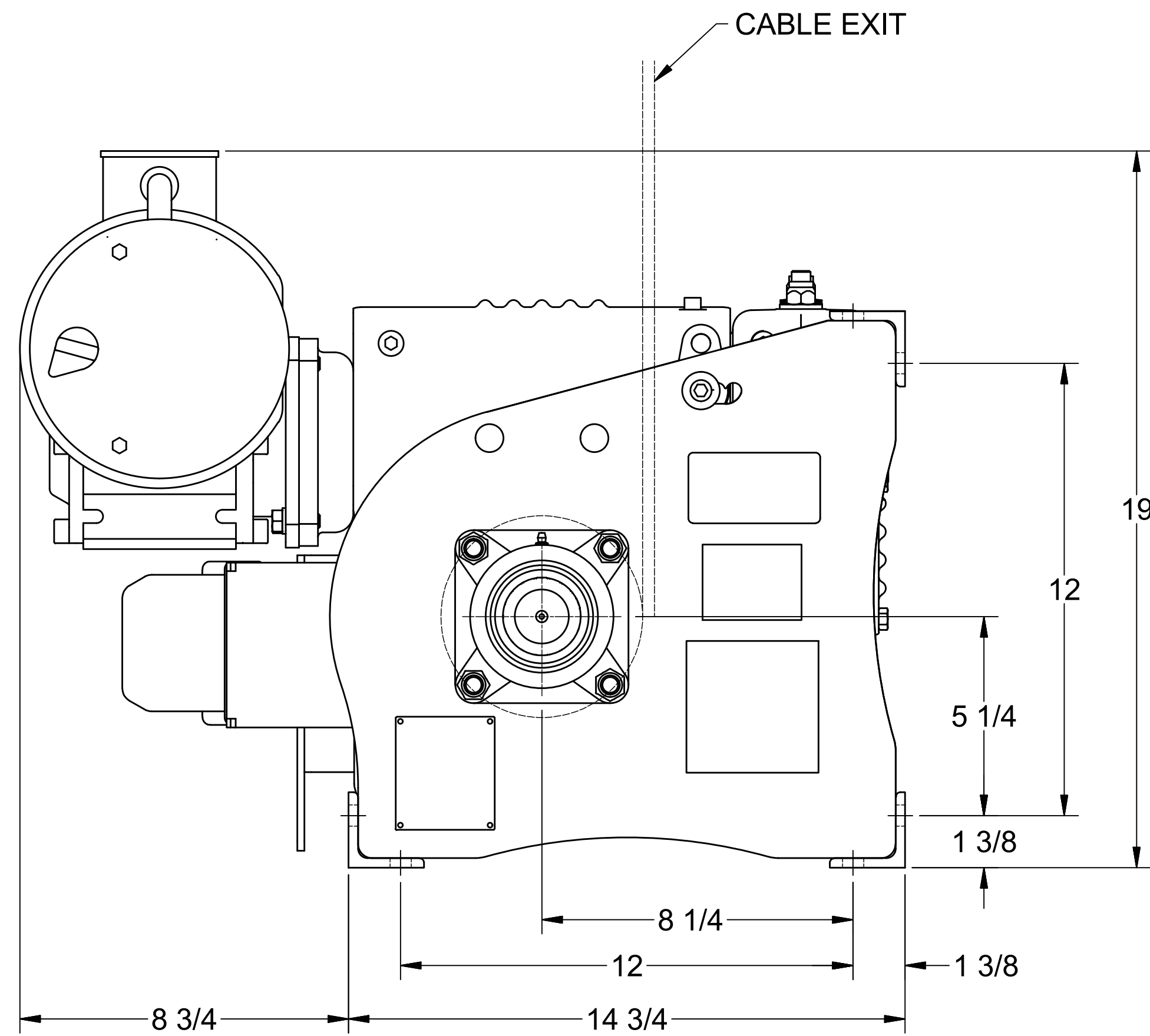
SIDE VIEW
