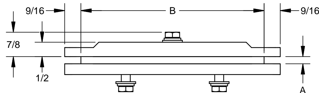
FB SERIES FLOOR BLOCK
